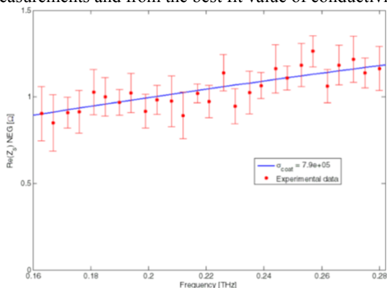
Figure 15: Surface impedance estimation of the 3.9 \mu m NEG coated slab: from averaged experimental data (red dots) and from best fit curve conductivity (blue).
