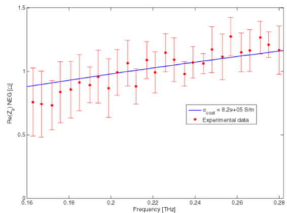
Figure 16: Surface impedance estimation of the 3.7 \mu m NEG coated slab: from averaged experimental data (red dots) and from best fit curve conductivity (blue).
